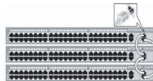
Figure 1b. Stackable Smart Switches are scalable and easy to manage. They can be easily stacked using connections on the front panel of the switch.
